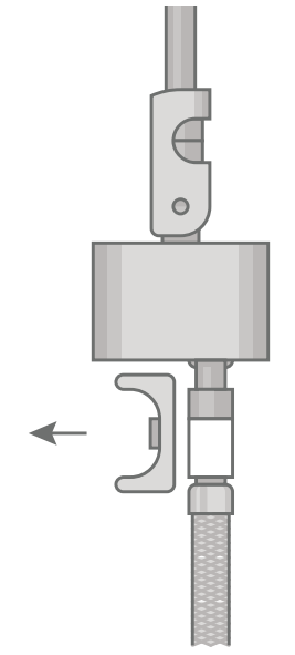
STEP 2. Remove the plastic clip from the bottom of your existing solenoid.
