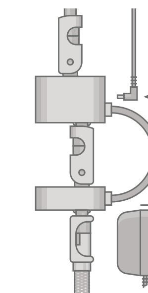
STEP 8. Connect the power supply to the solenoid and to an outlet that is not controlled by a switch. Reinstall SmartTouch® solenoid batteries* and turn on water supply.
